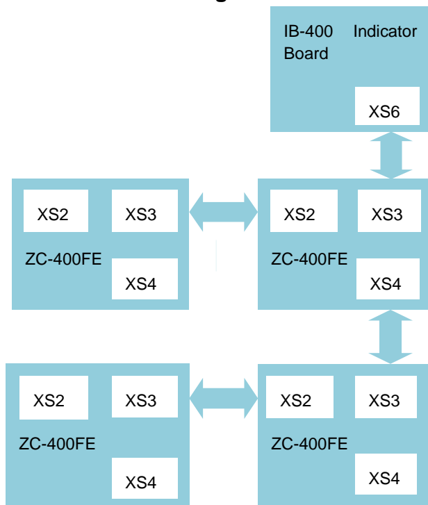
Fig. 1 Cascade Connection
