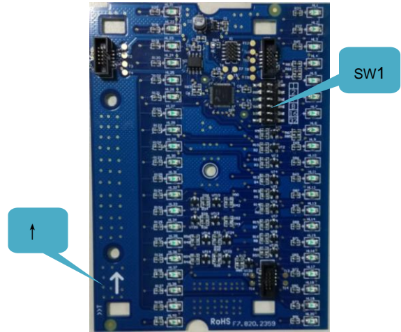
Fig. 2 ZC-400FE Zone Display and Control Board (RY color)
